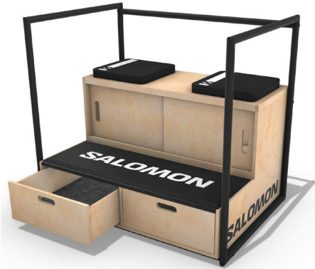
BENCH (L129,5CM / W 90.2CM / H 113.7CM) L47712400
